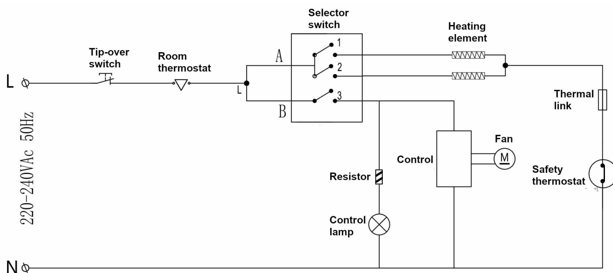
Wiring diagram CH 2100
